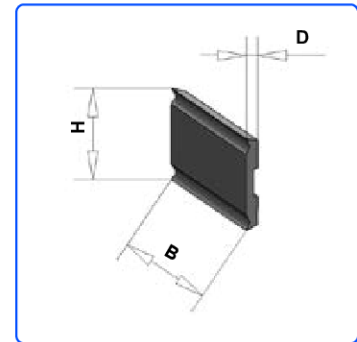
For System Versofix. With back groove TIN coated [1661]
