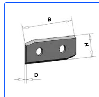
TOK with bevel, 2 cutting edges
