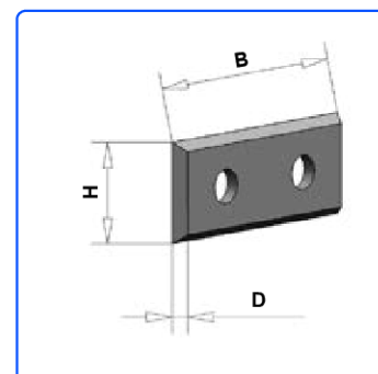
4 cutting edges (35°)
