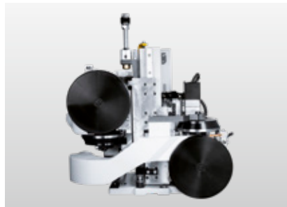
Multi scraper MN21 For smoothing trimmed edges to achieve an optimum appearance. Automatic resetting between max. 7 different profiles and corrections within the one-hundredth millimeter range. Reproducible quality to the highest standard.
