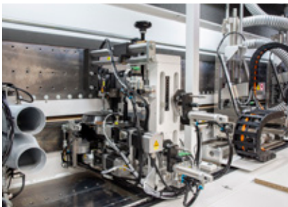
Profile scraper MN11 For smoothing the trimmed edges to achieve an optimum appearance. Automatic resetting between 2 different profiles. Fine corrections for reproducible quality at the highest level.
