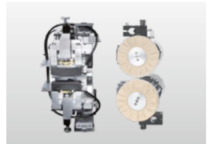
Finish processing Comprising a glue joint scraper for disposal of glue residues at the top and bottom of plastic edges and a buffing unit.
